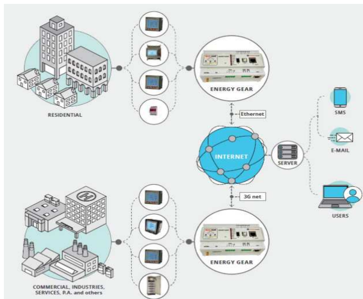
Datalogger gateway
